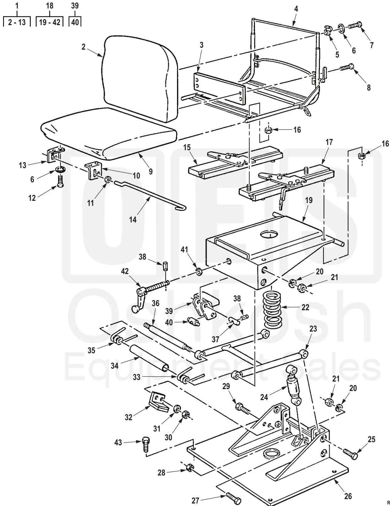
Figure 393. Operator's Seat Assembly.
